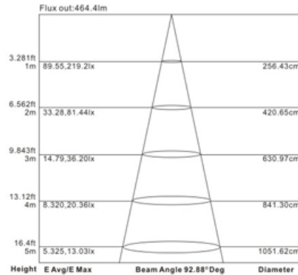
Note: The curves indicate the illuminated area and the average illumination when the luminaire is at different distance.
